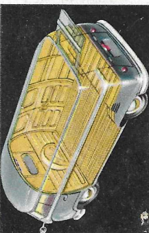
Loading capacity 170 cu. ft. — Payload 1830 lb.
